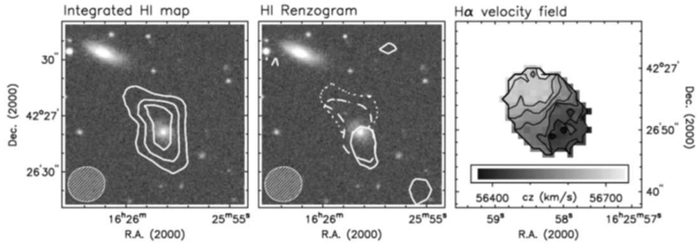
FIGURE 2. H I and H \alpha internal-velocity structure in a cluster galaxy at z=0.2 in A2192 (Verheijen 2004). H I data is typical of what can be achieved with today’s deepest surveys in advance of SKA-pathfinder facilities such as eVLA, ASAKP and MeerKAT. The H \alpha velocity-field was taken in 80 minutes on the Calar Alto 3.5m telescope using a 16x16 1” element integral field-unit of PMAS.
