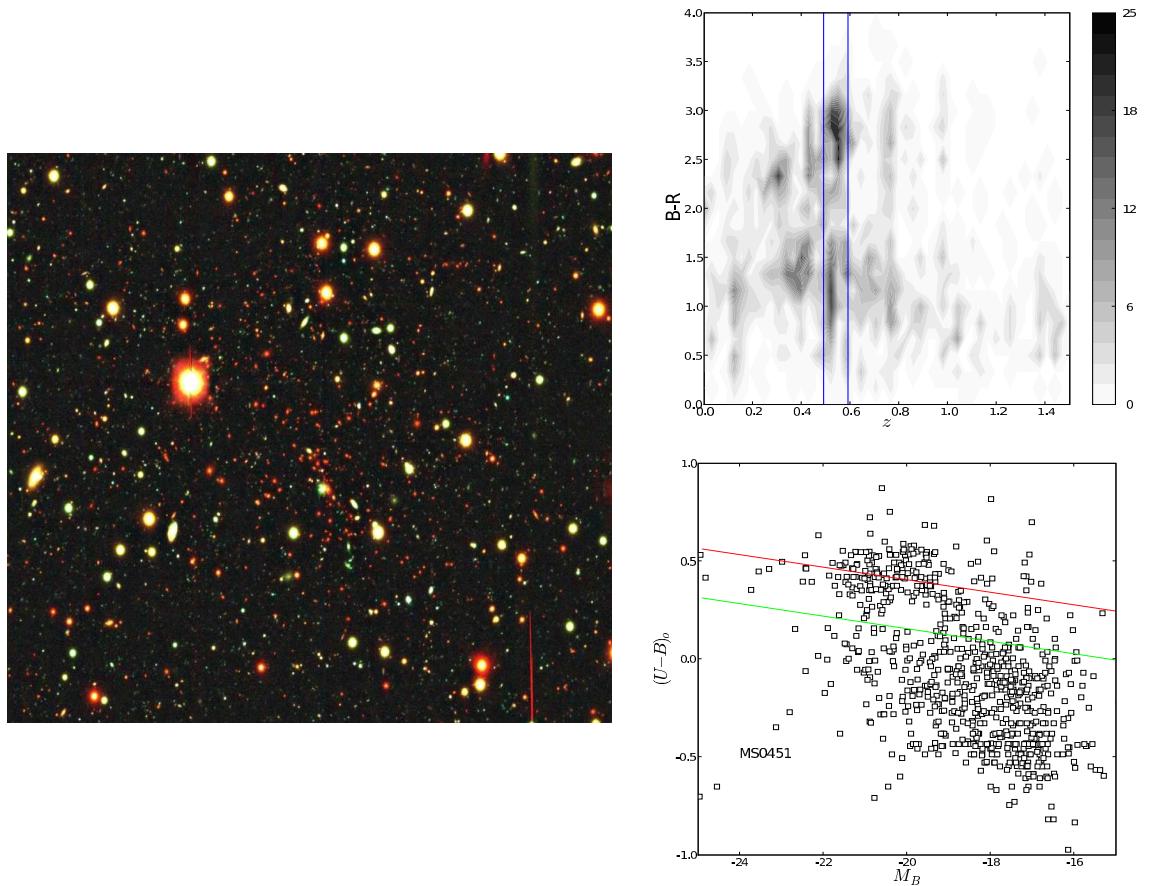
FIGURE 1. The blue cloud and red sequence in a deep field around MS0451, a rich cluster ( \sigma = 1354 \text{ km s}^{-1} and L_x = 40e44 \text{ ergs s}^{-1} ) at z=0.54 from the the WIYN Long-Term Variability Survey ( UBRIz bands, Crawford et al. 2006, 2008) The UBI 3-color image at left is a 10 \times 10 arcmin field. The corresponding B - R color-photometric-redshift diagram illustrates isolation of the cluster volume and the surrounding environment. The rest-frame U - B color-magnitude diagram shows the blue cloud and red sequence in this redshift slice. Data like these are at the upper-redshift limit of what could be well-probed with deep SKA-precursor HI surveys.
